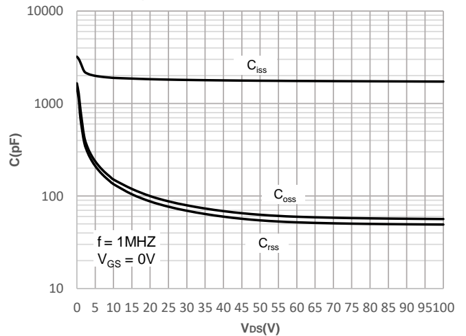
Figure 10: Capacitance Characteristics
